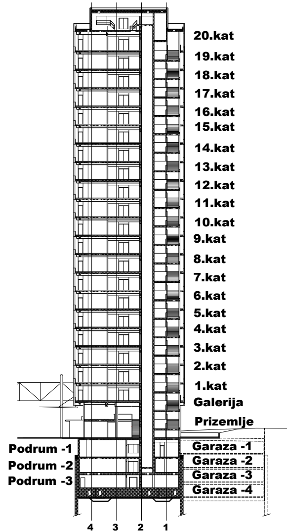
CROSS SECTION
