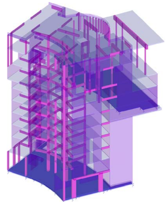
~ 3D MODEL (MIDDLE DILATATION)
