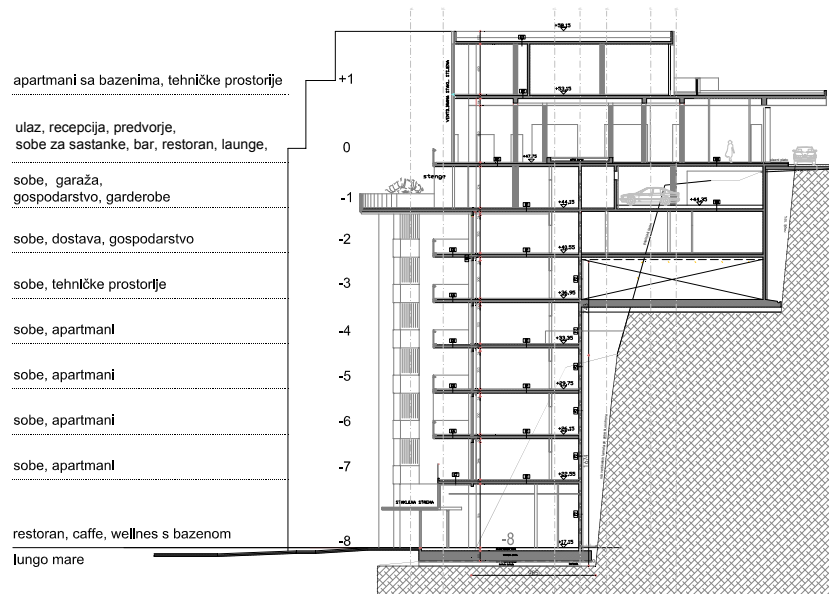
~ CHARACTERISTIC CROSS SECTION
