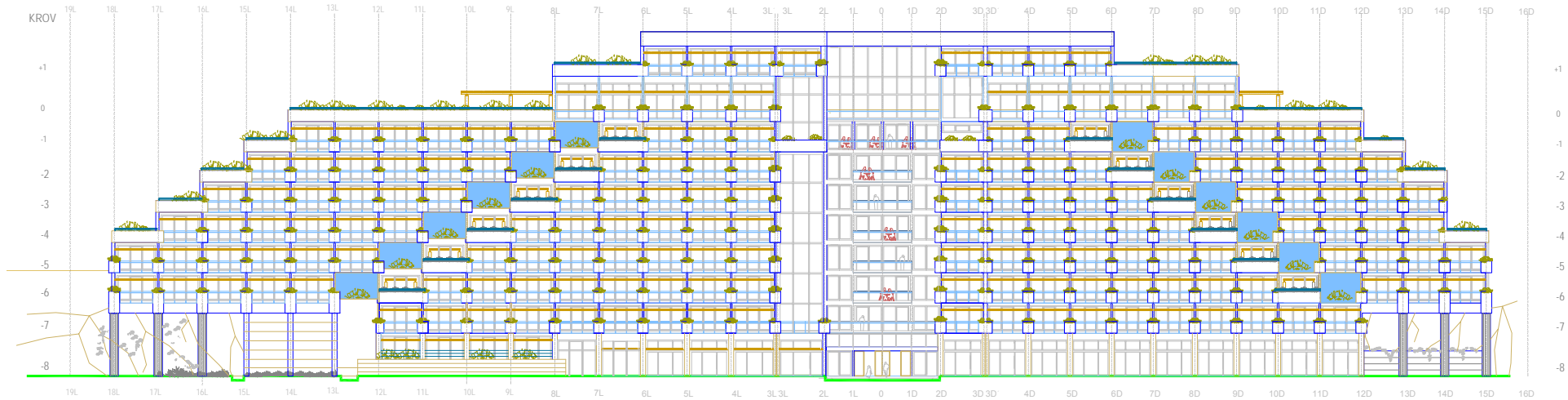
~ SOUTH FACADE
